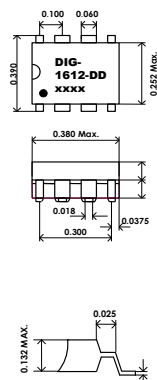
8ld Pdpip Gull-wing
